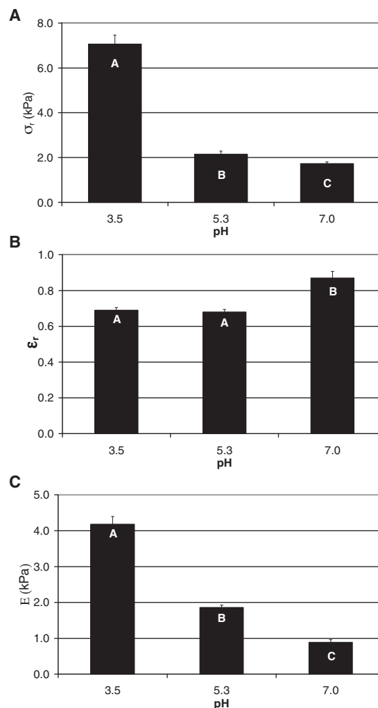
Fig. 4. Mechanical properties of gels of 1.5% (w/w) gellan gum at pH 3.5, 5.3 and 7.0. (A) Stress at fracture ( \sigma_I ), (B) strain at fracture ( \epsilon_I ) and (C) Young's modulus ( E ). Means and error bars were calculated from triplicates of each sample. Means with different letters show statistically significant differences at p < 0.05 .
